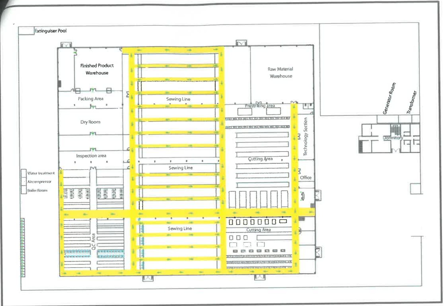
Figure 2: Factory Layout Plan
