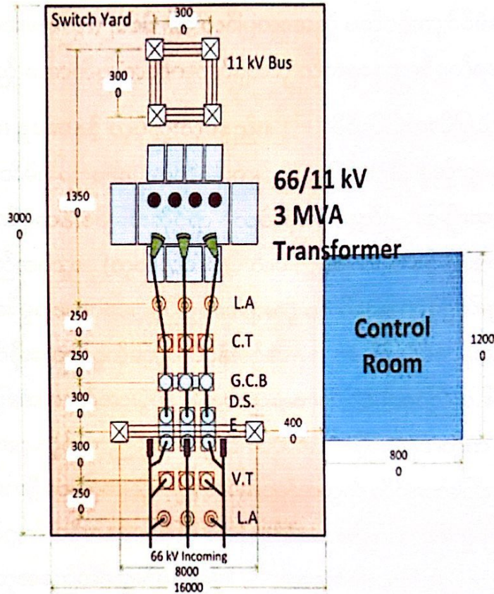
Lay Out Plan of Sattwar(Taungdwingyi)66/11 kV,3 MVA Sub-Station
