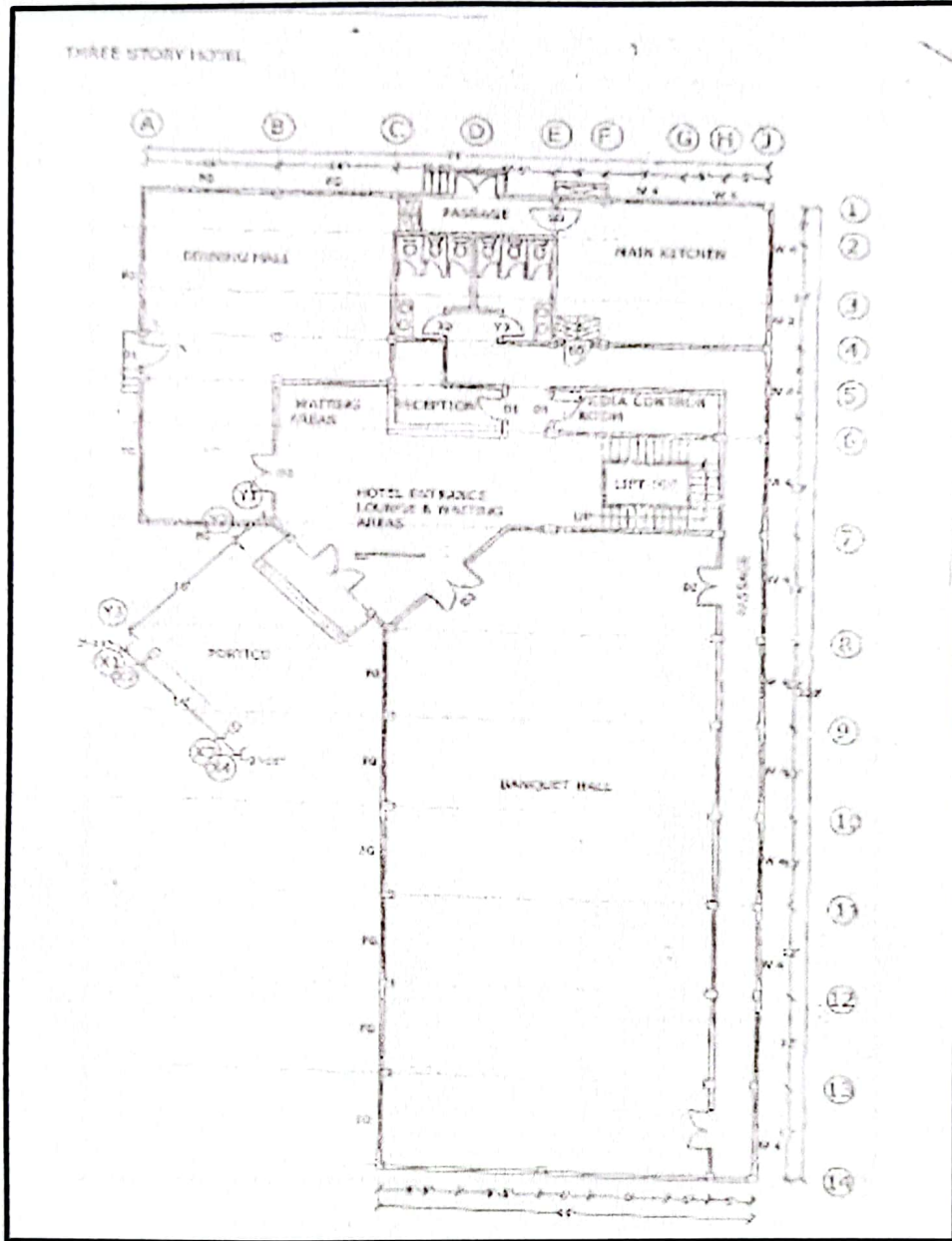
Figure 2: Ground Floor Layout Plan of Golden River Hotel
