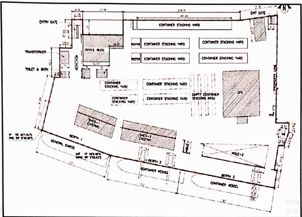
Figure 2: Layout Plan of TMT Ports
