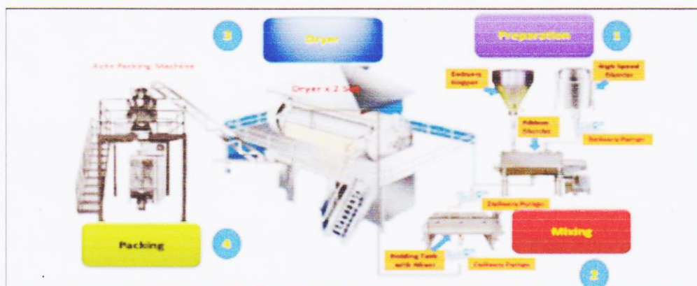
Figure 3: Cereal Flakes Production Process Block Diagram
