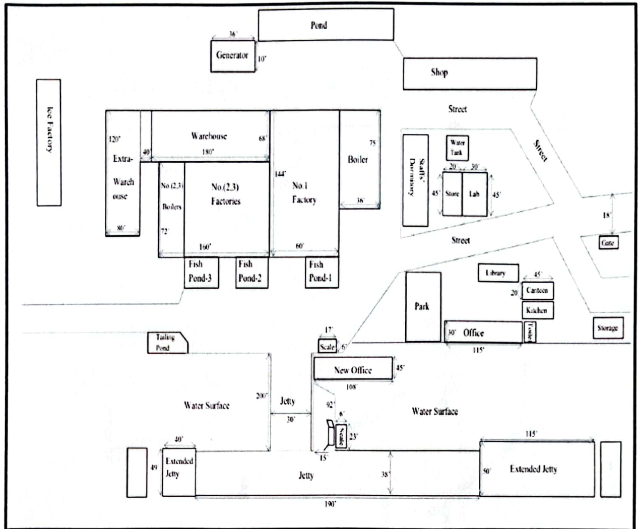
Figure 2: Layout Plan of the Fishmeal Powder Factory
