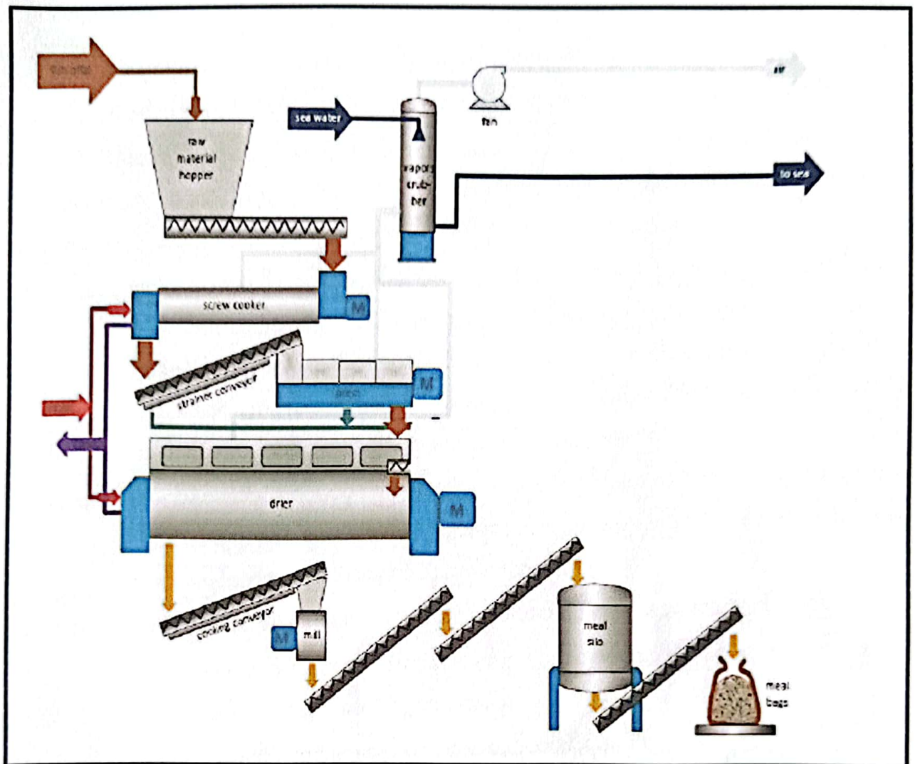
Figure 3: Flow Diagram of Fish meal Powder Process
