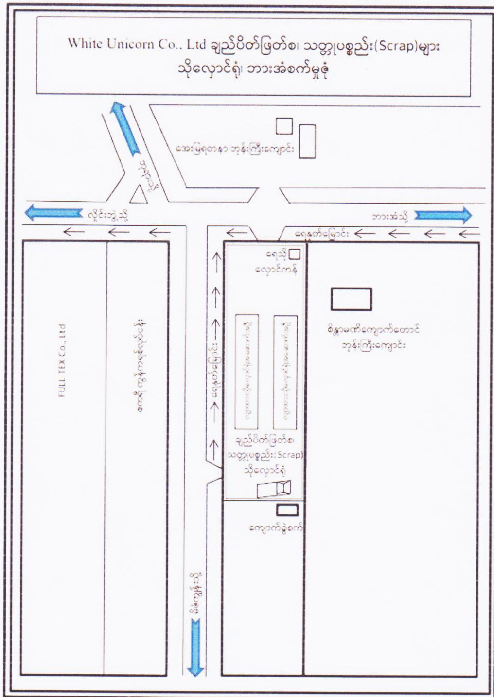
Figure 2: Layout Plan
