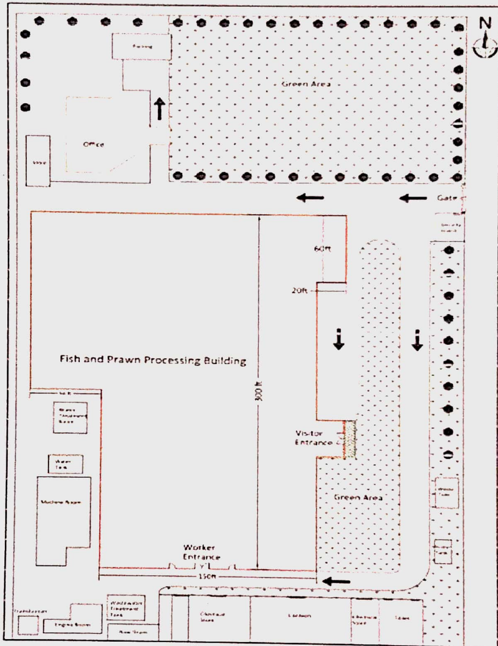
Figure 2: Layout Plan
