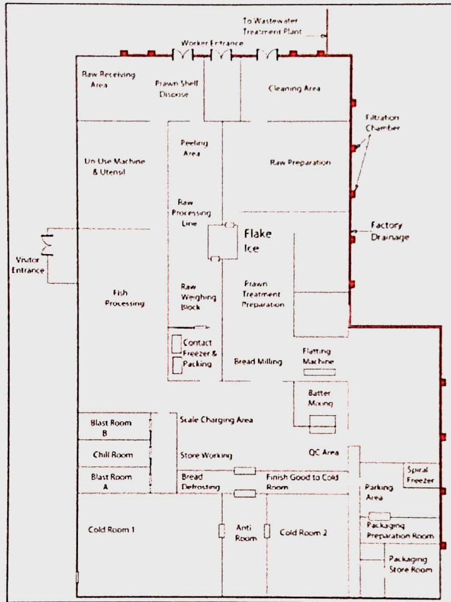
Figure 3: Wastewater Treatment Layout Plan
