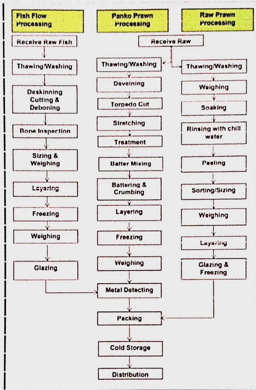
Figure 4: Fish and Prawn Processing Flow
