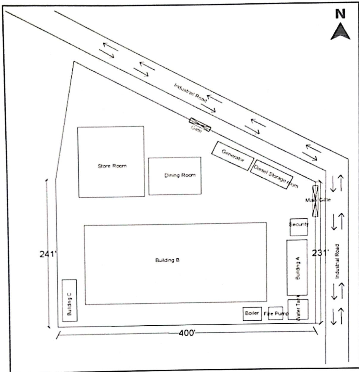
Figure 2: Factory Layout plan
