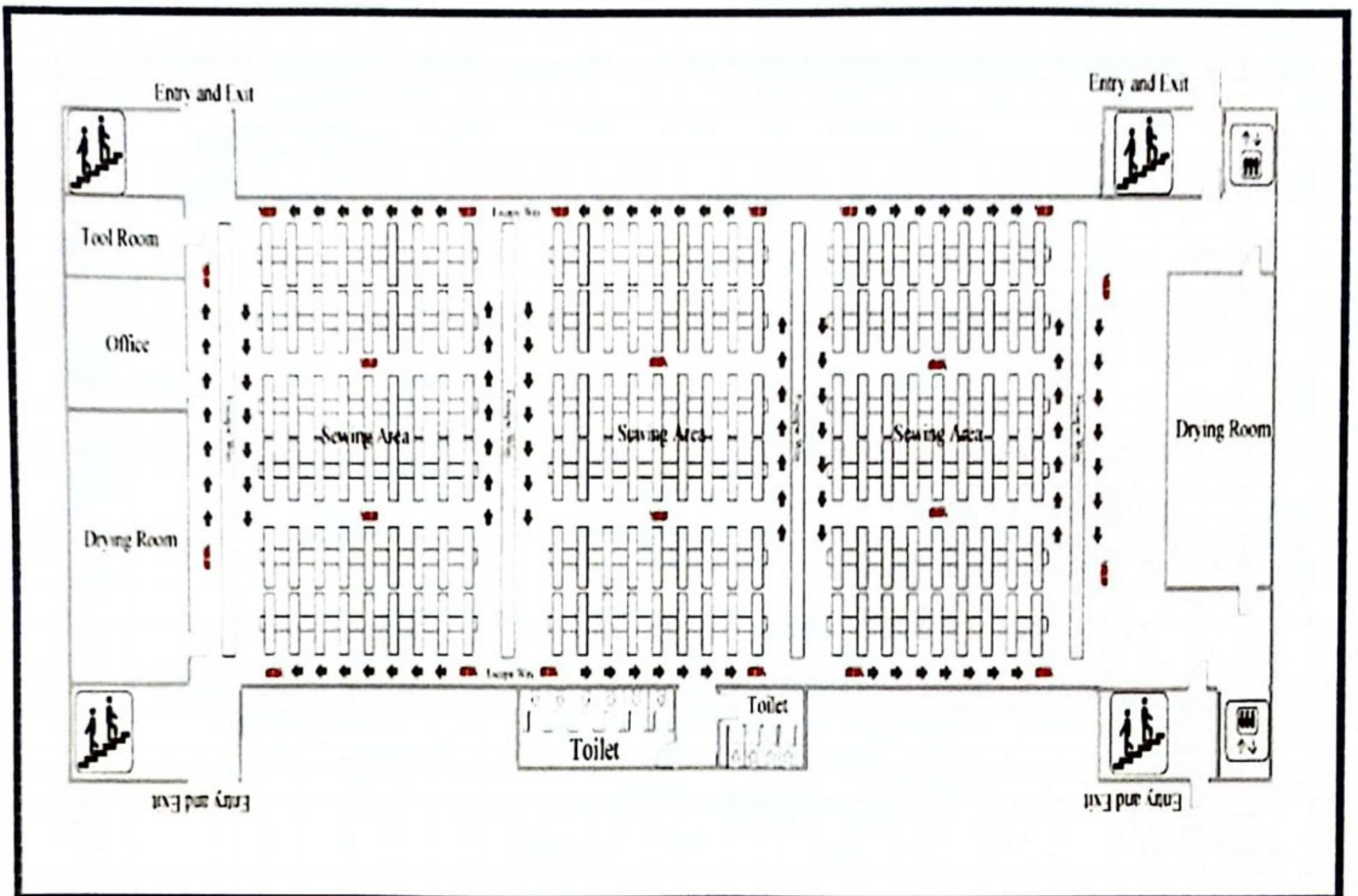
Figure 3 : Factory Layout Plan
