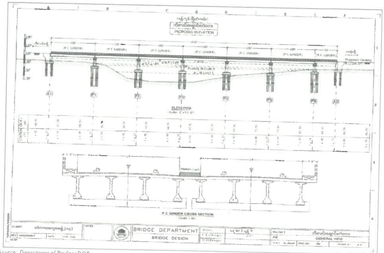
Figure 3 : Layout Design of Bridge
