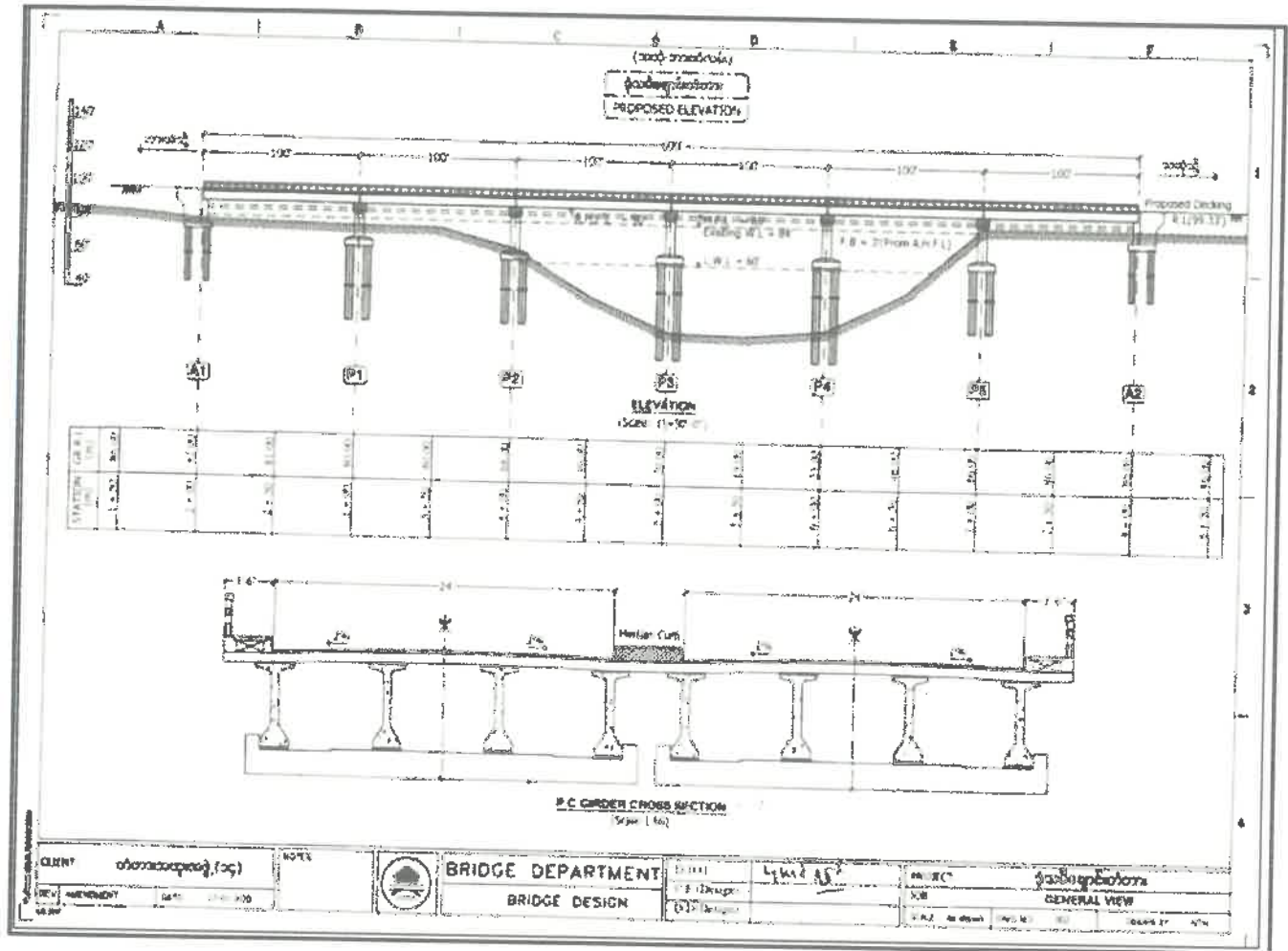
Figure 2: Engineering Design For Proposed New Donthami Bridge
