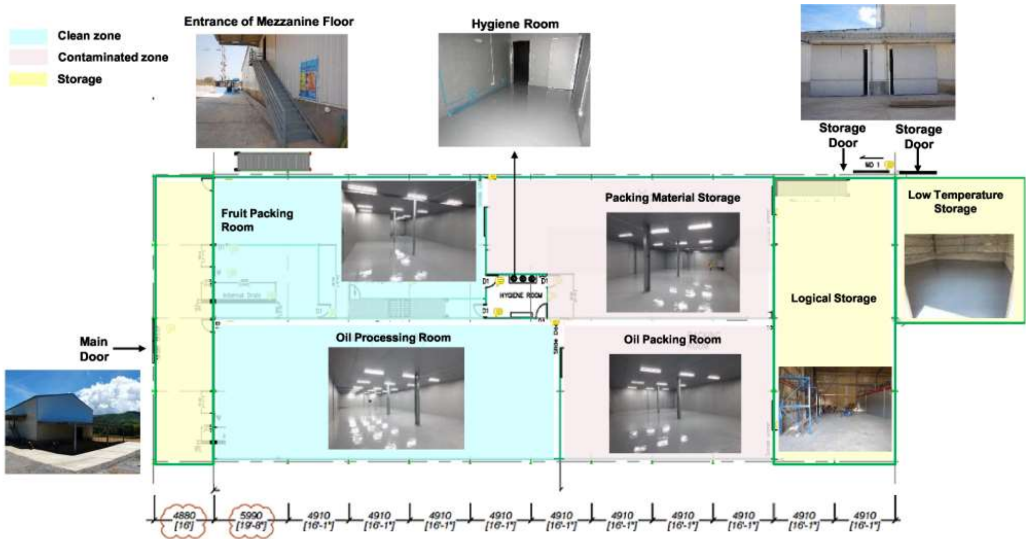
Figure 4: Layout for ground floor
