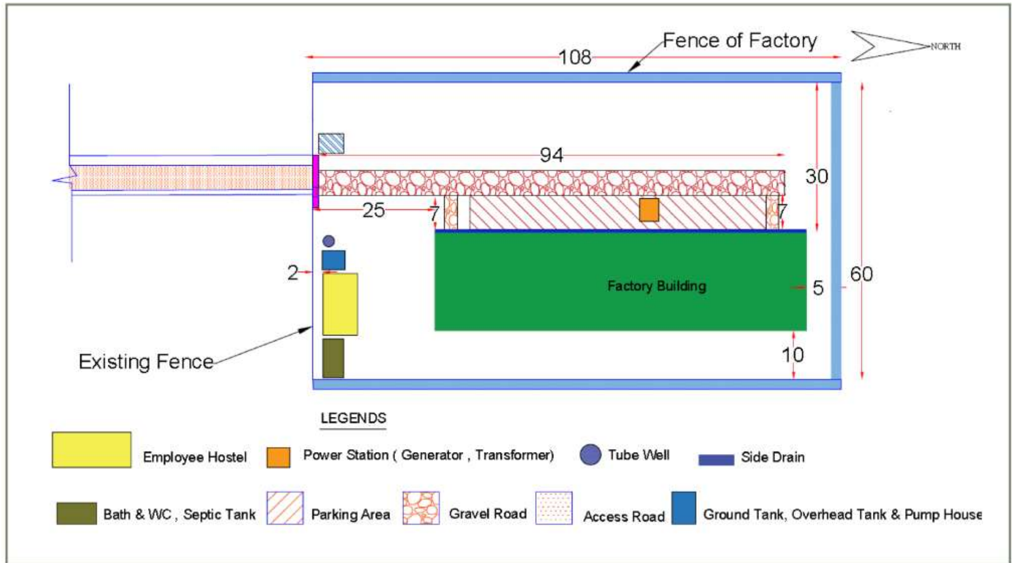
Figure 3: Factory Building Layout
