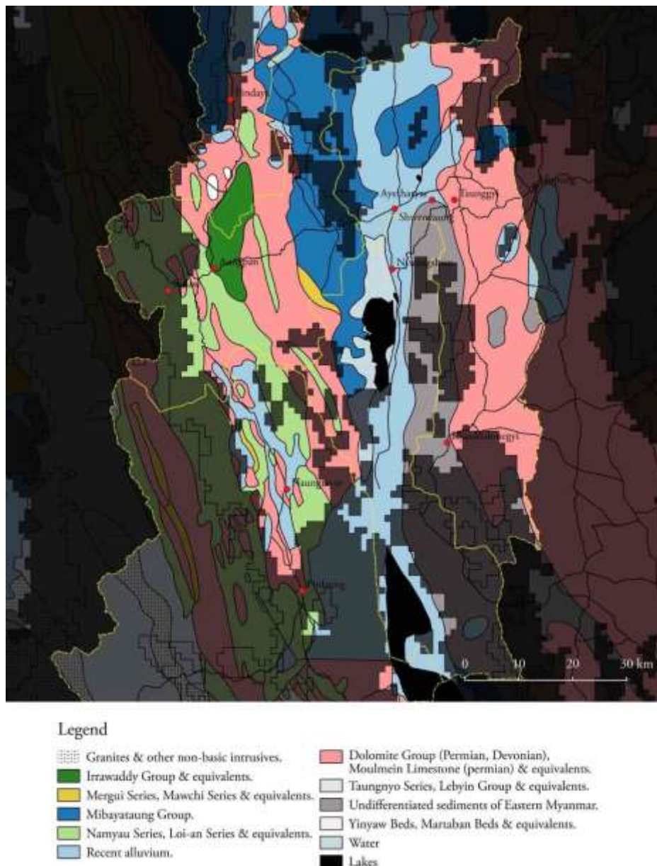
Figure 25: Latest geological map
