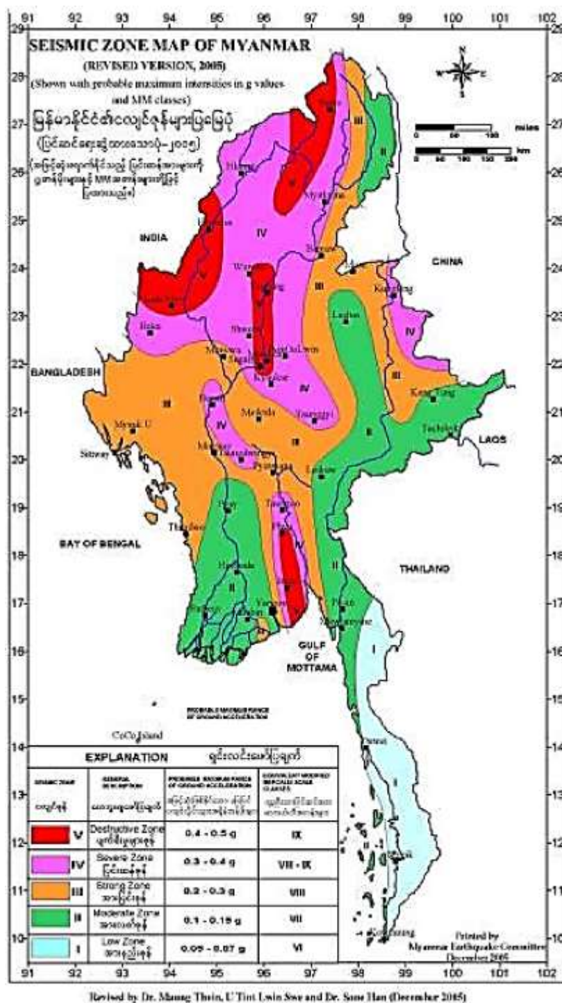
Figure 26: Seismic zone map of Myanmar
