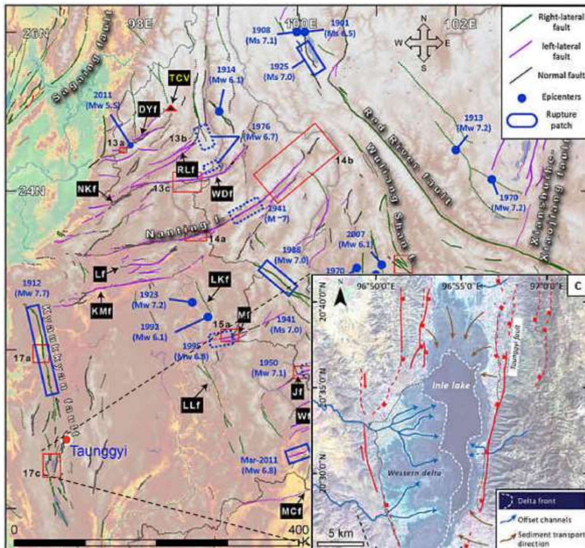
Figure 27: Fault zones within area of interest
