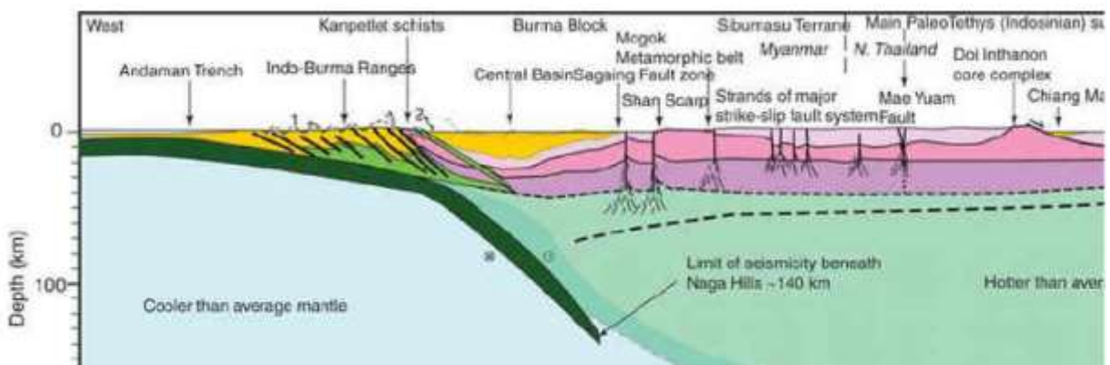
Figure 24: Geological cross-section of Myanmar
